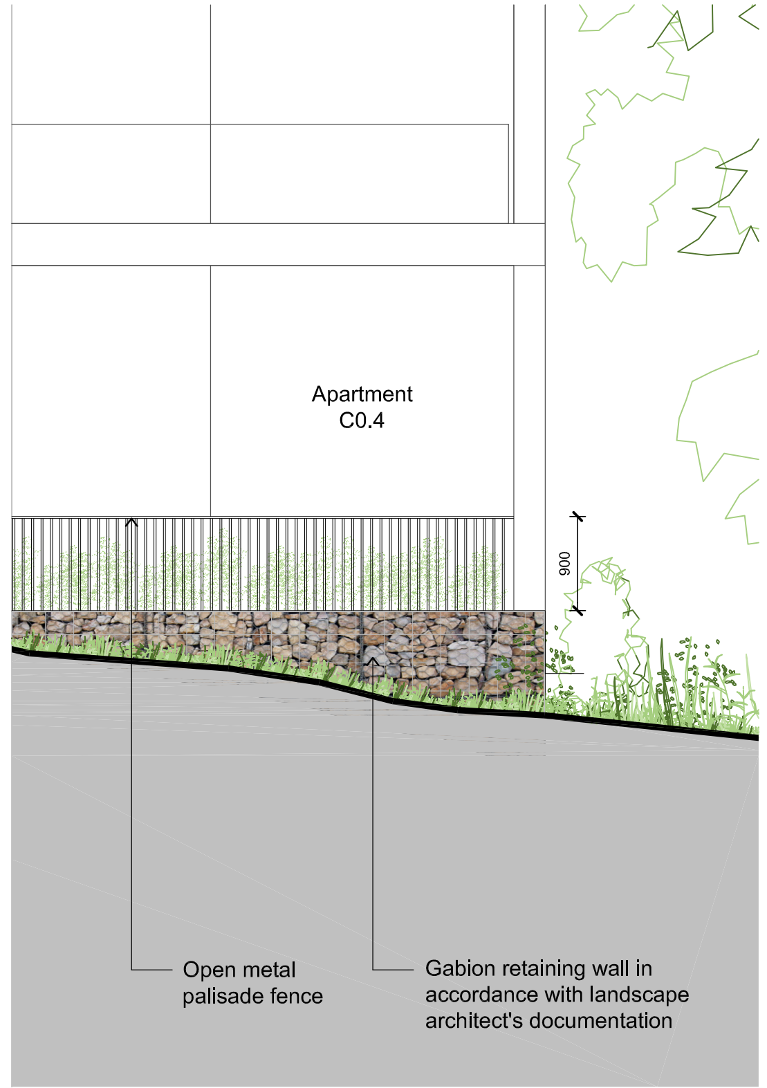
3 Typical Elevation of Garden Fence Looking North Building C 1:50 @ A1
